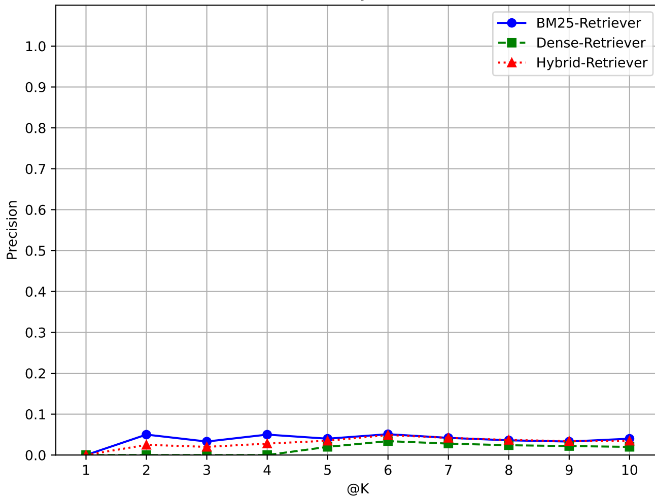
Query 32
